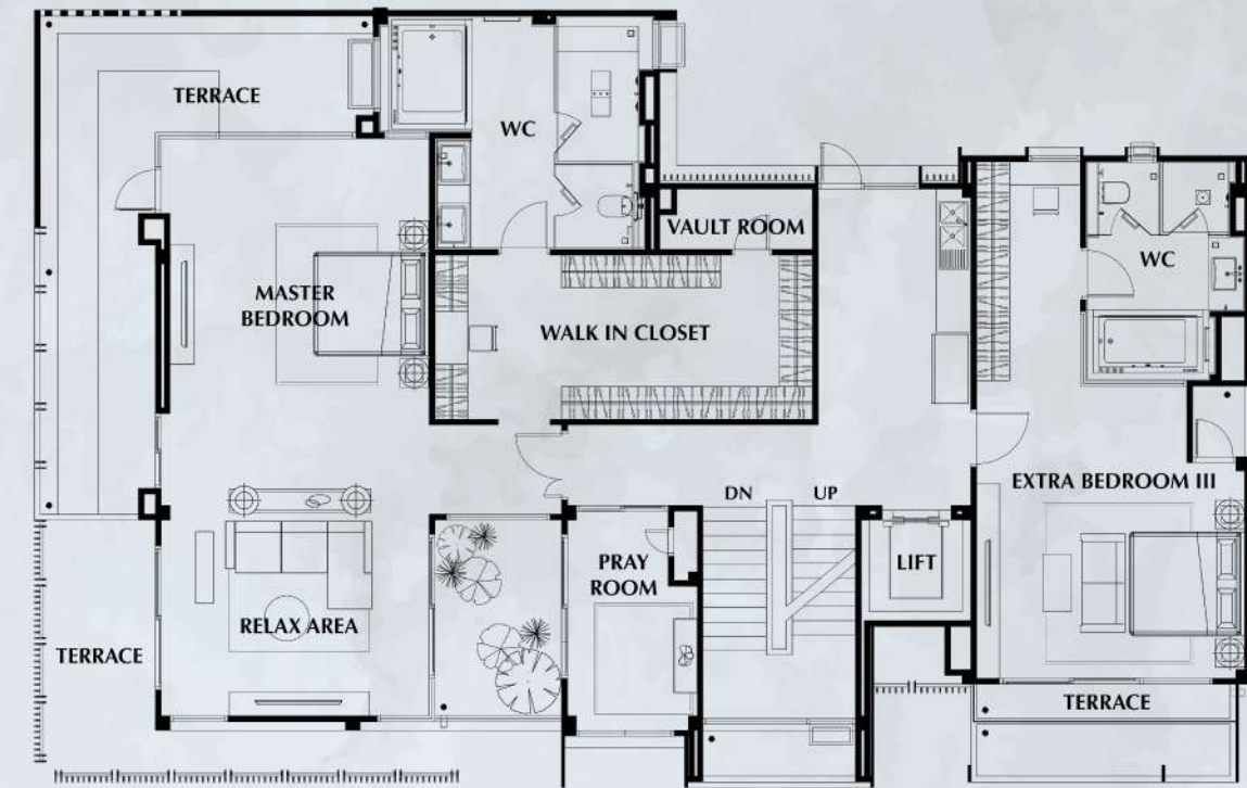
3 rd FLOOR
